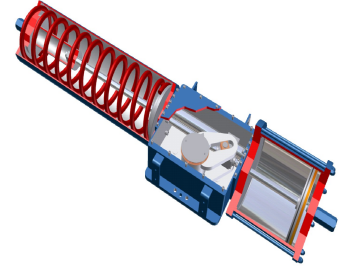
Figure 2. PN pneumatic scotch yoke actuator final assembly
